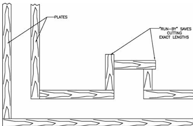
Typical Plate Configurations
