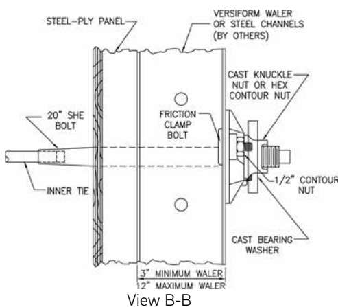
Cast Bearing Washer and She-Bolt Detail
