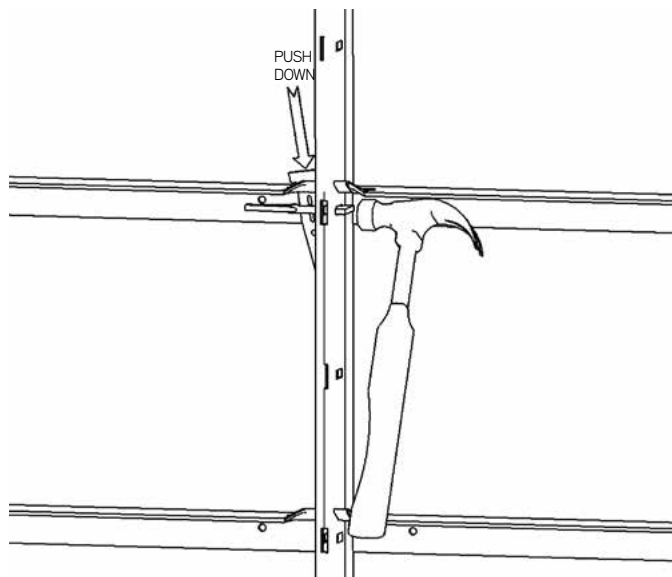
Hammer Strikes Horizontal Wedge Bolt
