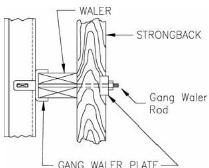
Water and Strongback Attachment with Gang Waler Plate
