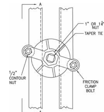
Cast Bearing Washer and Taper Tie Detail
