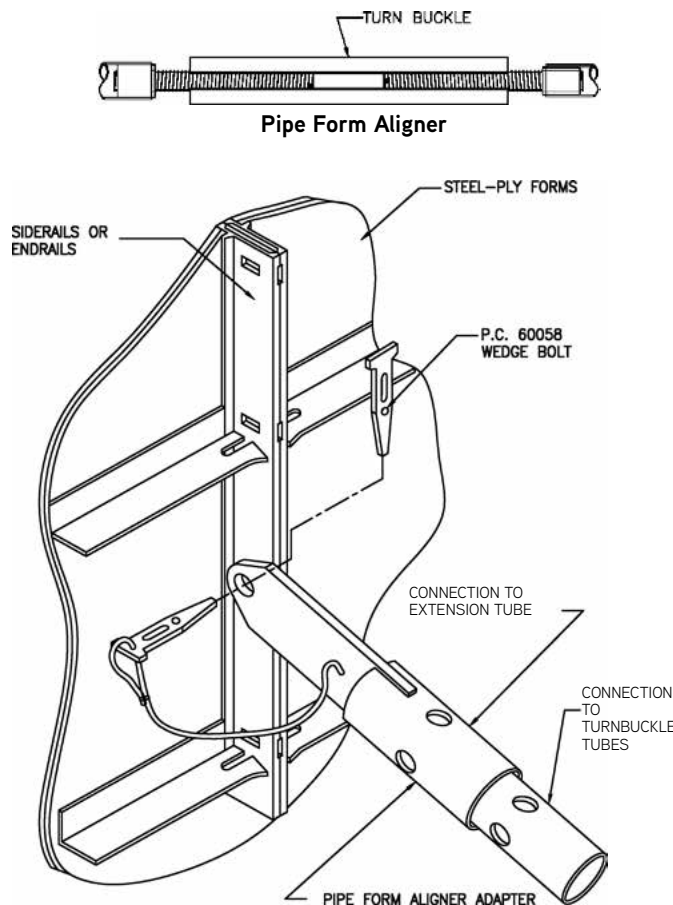
Pipe Form Aligner Attachment to Steel-Ply
