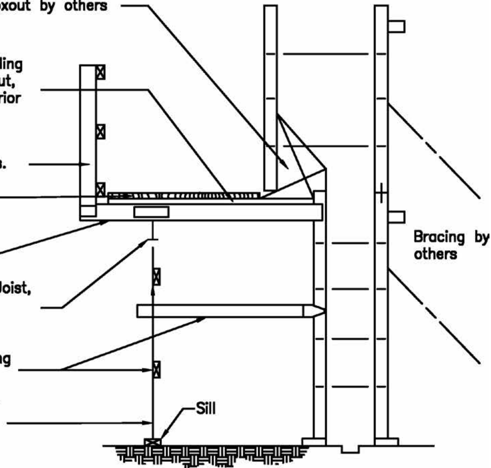
Typical Haunch Support Bracket Application
