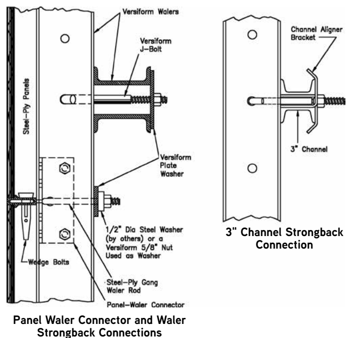
Section View
