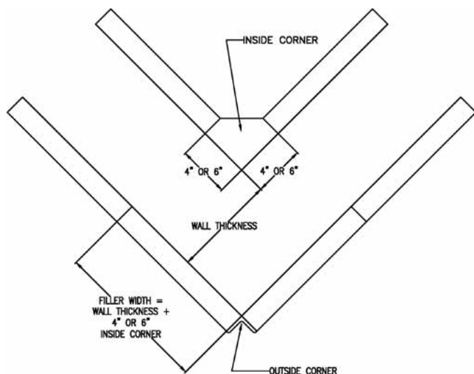
Typical Start Point for Panel Erection
