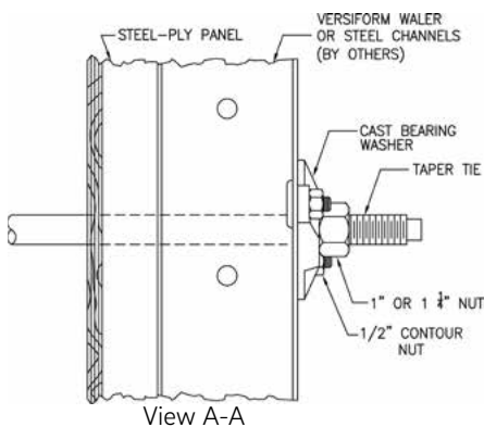
Cast Bearing Washer and Taper Tie Detail
