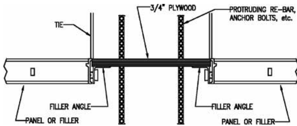
Typical Job-Built Filler with Rebar Penetrations
