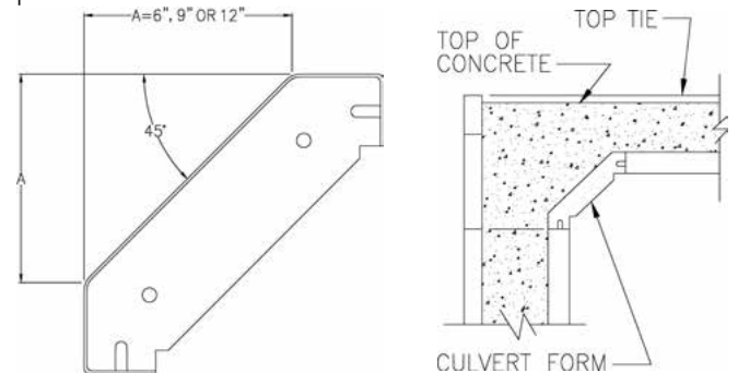
Culvert Form Angle
