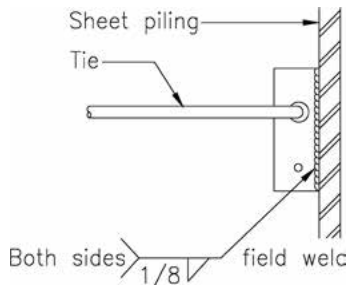
Single End Threaded Toggle Tie Application #1
