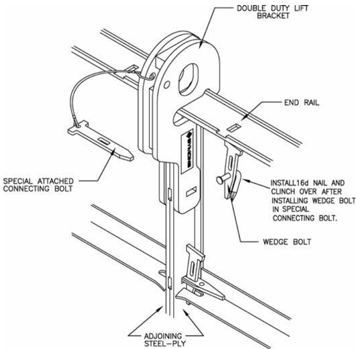
Double-Duty Lift Bracket Installation
