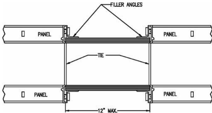
Typical Job-Built Filler with Filler Angles
