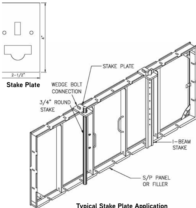
Typical Stake Plate Application
