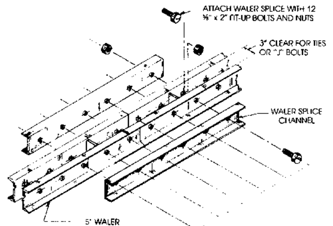
Waler Splice Angle Installation
