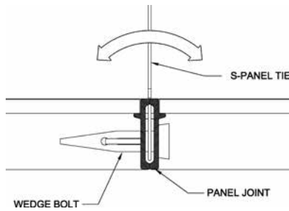
Lateral Swing of Panel Tie
