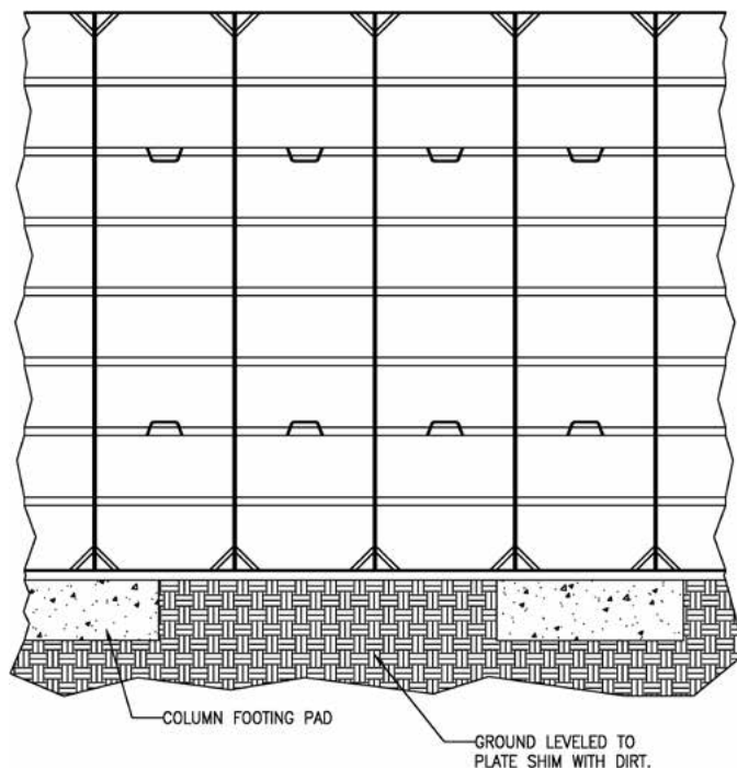
Typical Plate and Footing Pad Configuration
