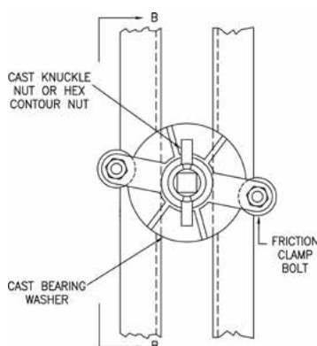
Cast Bearing Washer and She-Bolt Detail
