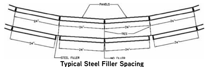
Typical Steel Filler Spacing
