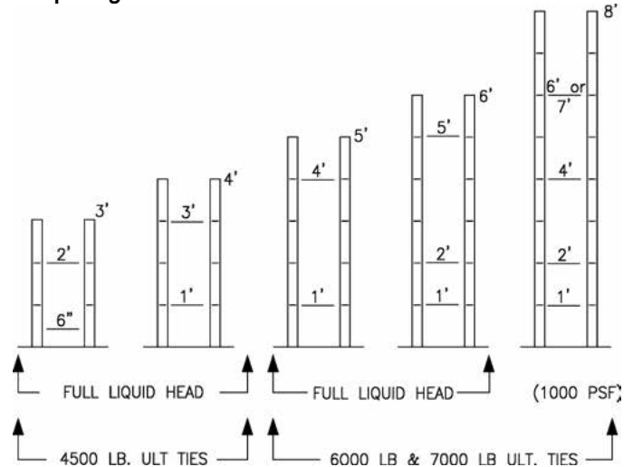
Tie Spacings Walls 8' Tall or Less
