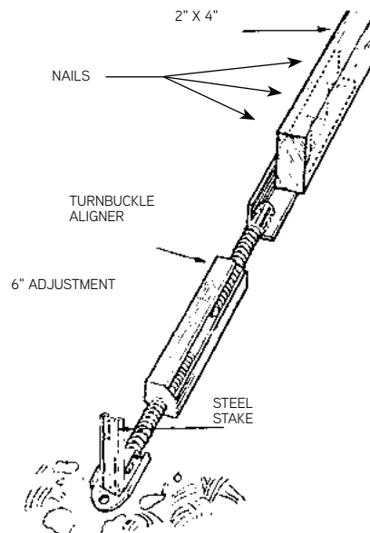
Typical Turnbuckle Aligner Application
