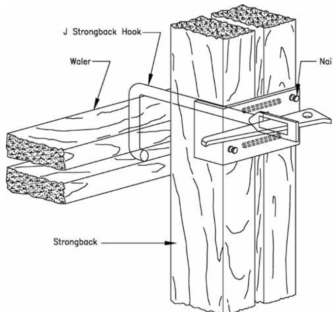
Typical Strongback Connection to Waler with J-Strongback Hook
