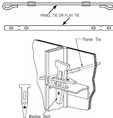
Typical Wedge Bolt Connection through Ties and Side Rails
