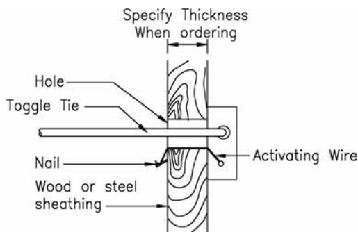
Single End Threaded Toggle Tie Application #2
