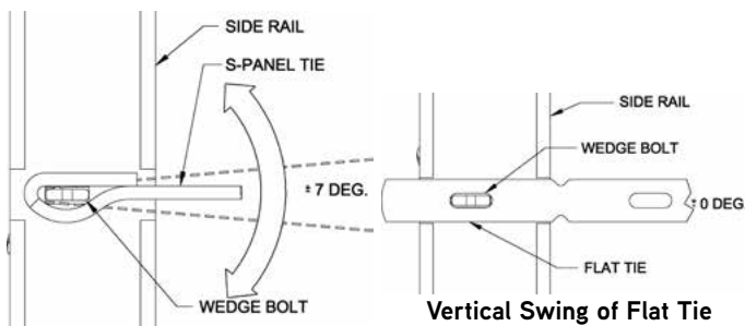
Vertical Swing of Panel Tie
