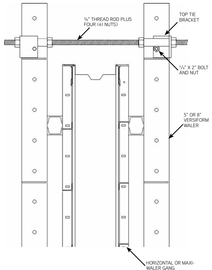
Typical Adjustable Top Tie Installation
