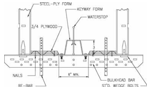
Keyway Bulkhead
