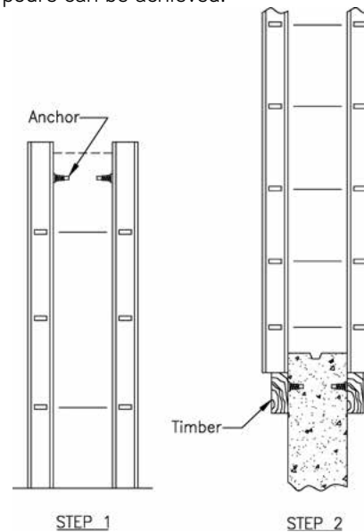
Second Lift with Supporting Lumber
