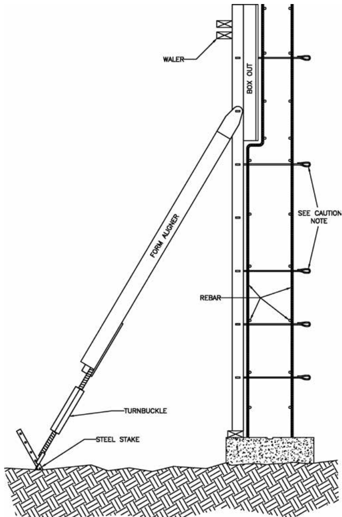
Typical Alignment Brace Installation
