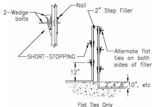
Typical Step Forming with Flat Ties
