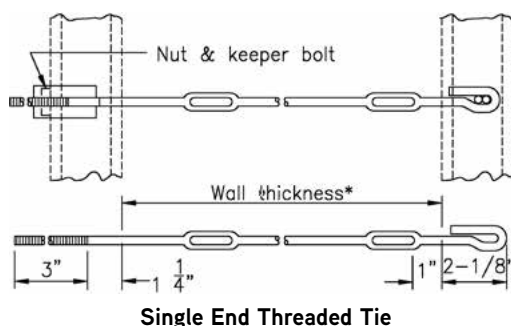
Single End Threaded Tie
