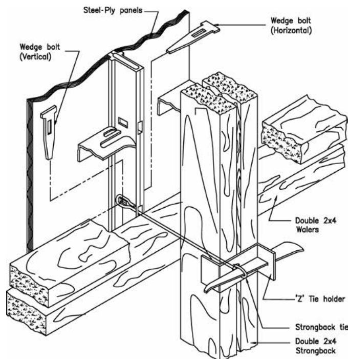
Typical Strongback Installation with Strongback Tie and Z-Tie Holder
