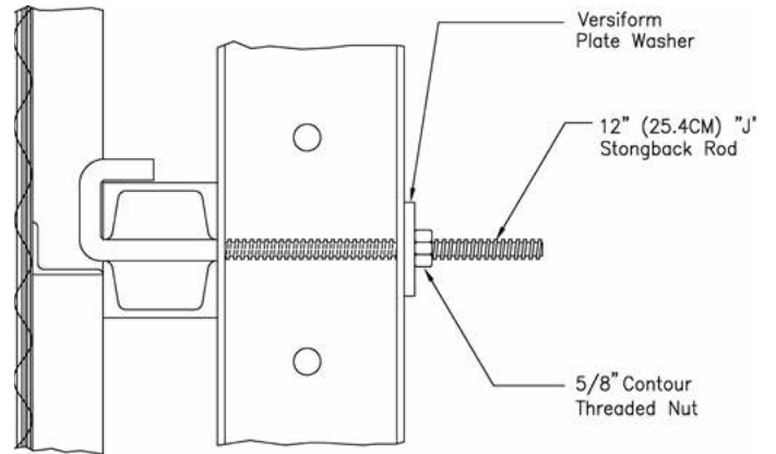
View B-B
